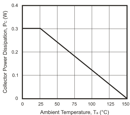
Fig.8 - P_C — T_a
