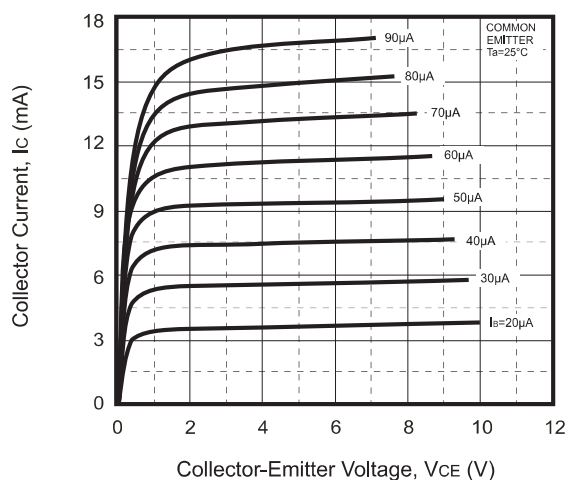
Fig.1 - Static Characteristic
